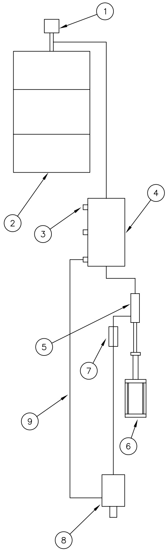
SYSTEM LAYOUT, CMP SINGLE METER
